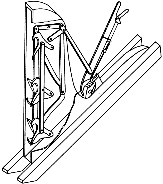
Figure 8-15. Boss dog.
